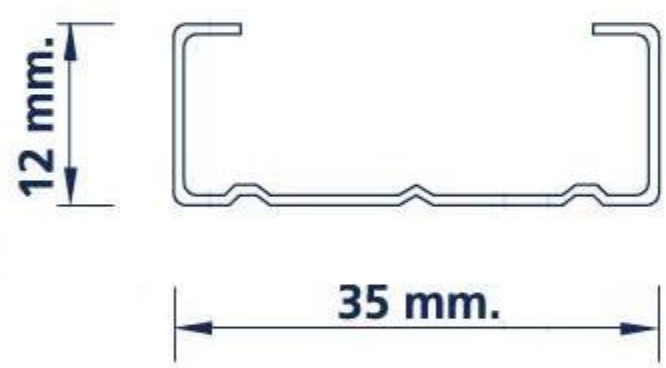
SL40 Channel
