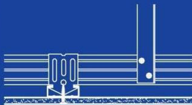
Screw Fixing SL40 channel with SA1 Steel Angle (Hanger)
