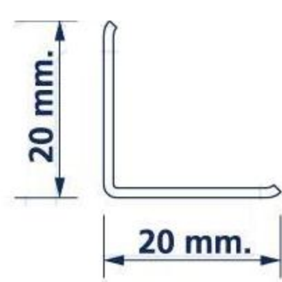
SA1 Steel Angle
